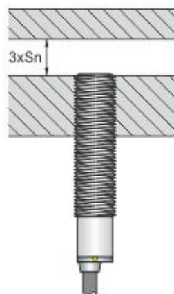
Flush mounting
