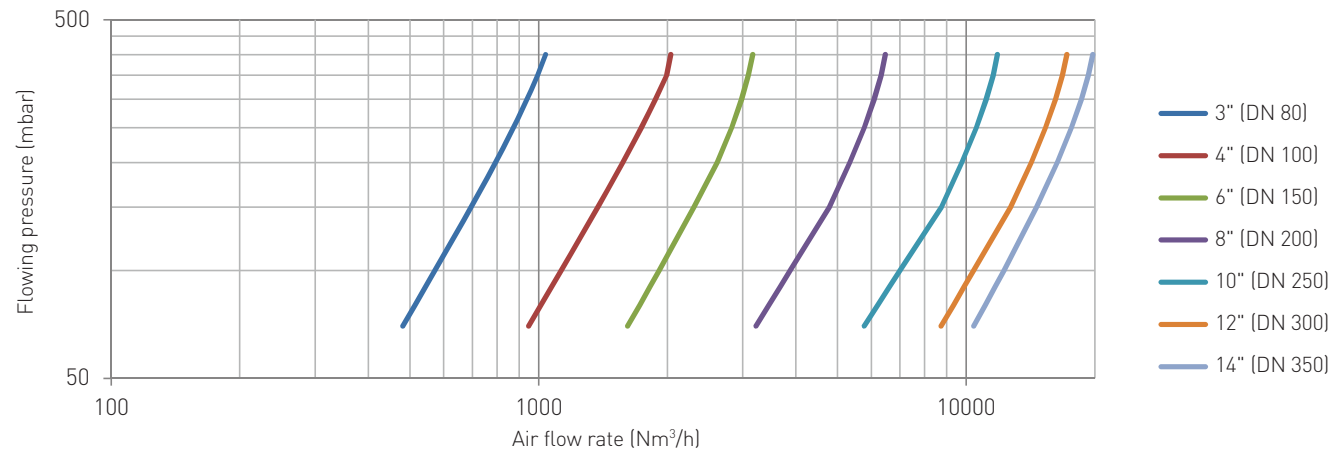
4410HV [Conical reducer]
