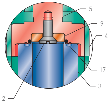
83 SEAT (O-RING)
