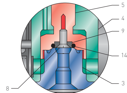
83 SEAT (O-RING)
