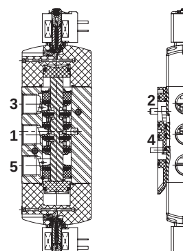
bistable (553 Series)
