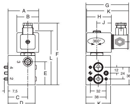
TYPE 03: Metal, epoxy coated / AISI 316L SS WP / WS: IEC 60335-1 EM / WSEM: EN/IEC 60079-7+18+31
