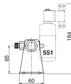
Supply rail with isolation valves for series 551
