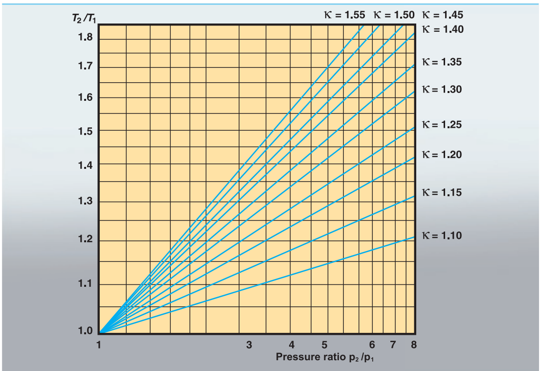
Diagram showing the temperature ratio T_2/T_1 for different gases having different K -values during isentropic compression.
