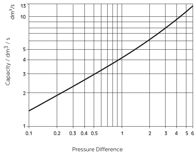
Discharge Capacity
