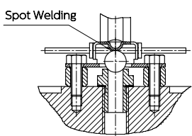
C-C Cut View
