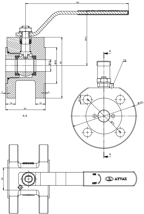
DN20 MBK-45 Monoblok Valve Dimension
