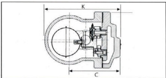
THREADED CONNECTION
