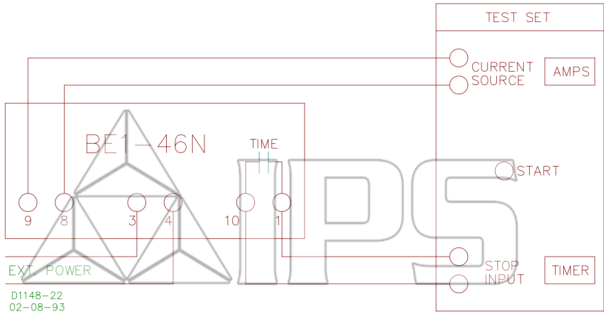
Figure 5-1. Test Setup Diagram
