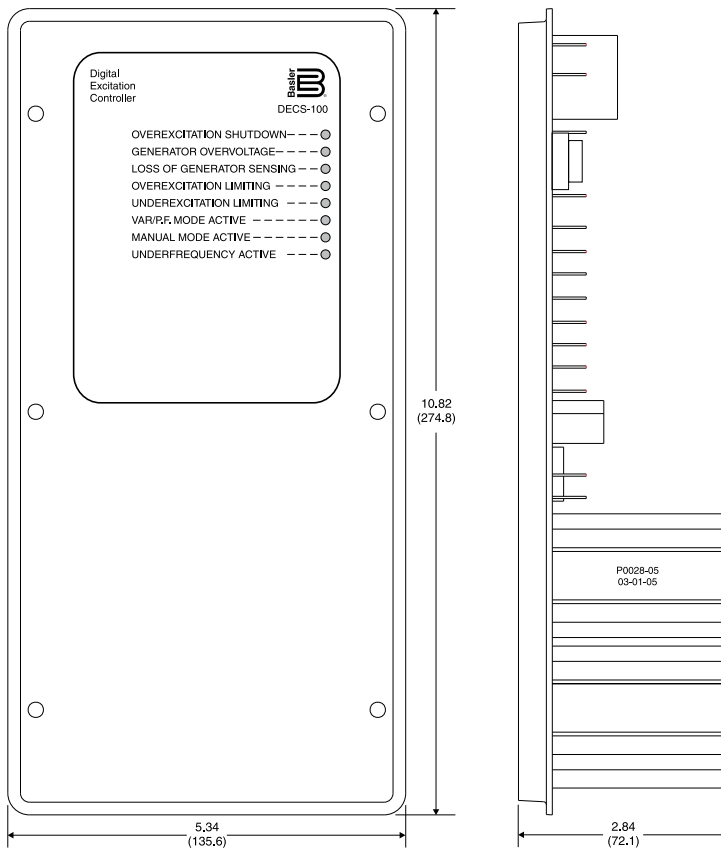
Figure 3 - DECS-100 Dimensions
