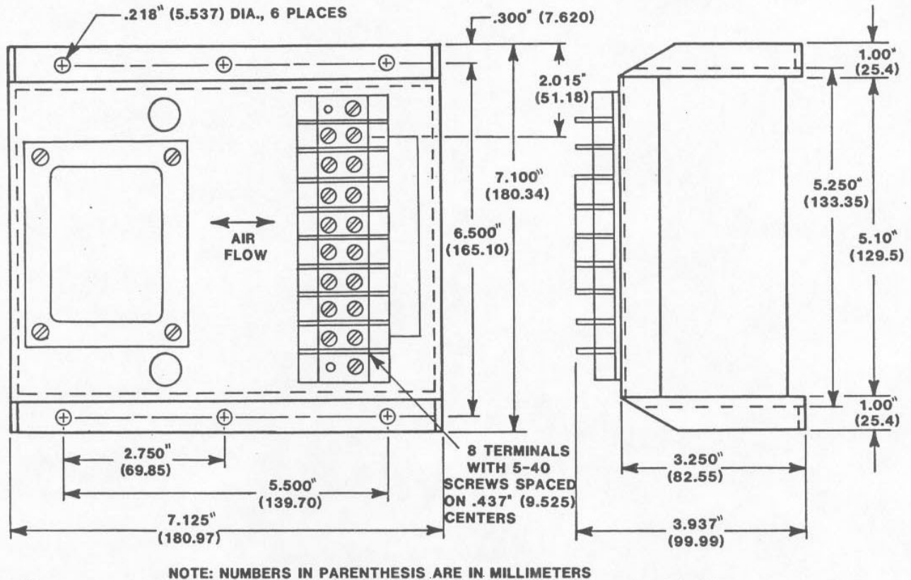
Figure 4-3. Outline Drawing.
