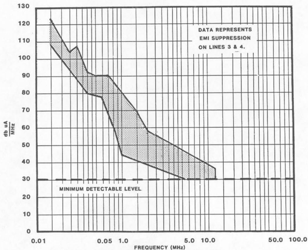
Figure 1-1 Typical Suppression of Conducted EMI
