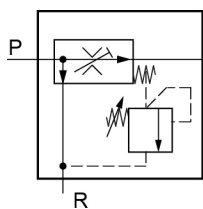
3-way flow control valve Priority flow is fixed Pressure relief valve for P
