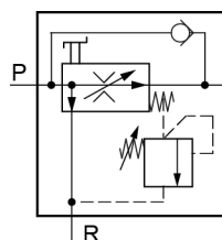
3-way flow control valve Priority flow is adjustable by handwheel Pressure relief valve for P Bypass check valve from A → P
