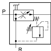
3-way flow control valve Priority flow is adjustable by handwheel Pressure relief valve for P
