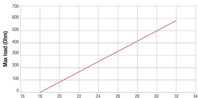
Maximum load on current loop
