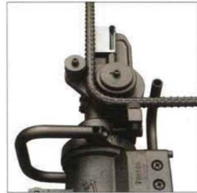
Bending 90°
