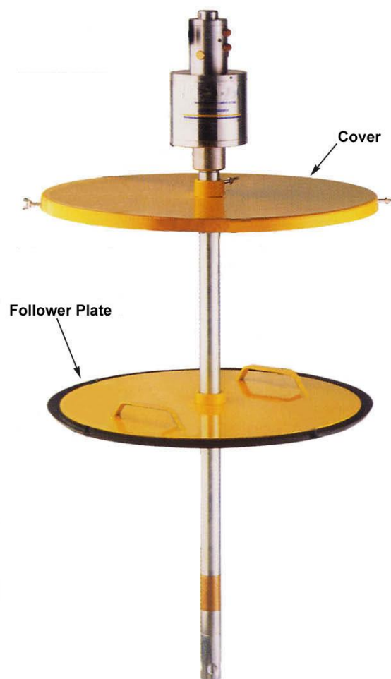
Pump with cover and follower plate
