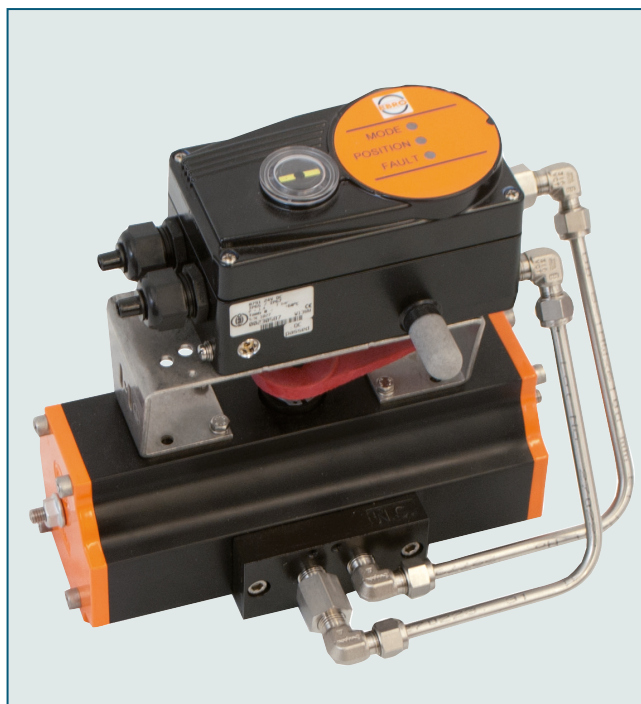
Basic version (EP 501-B) without a digital display. Stainless steel piping on request.
