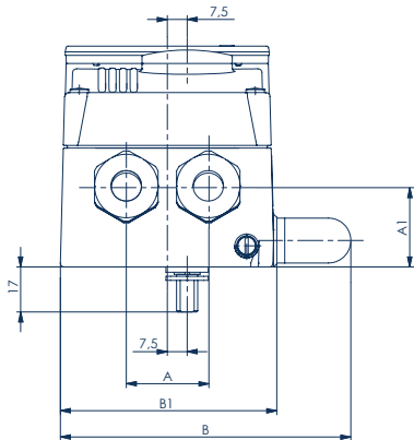
Standard EP501 (R)
