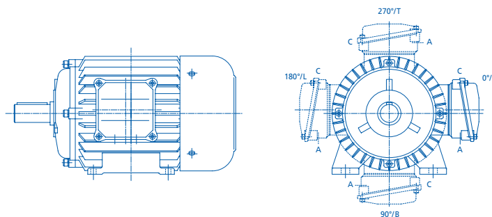
Terminal box position
