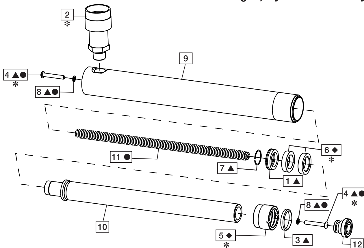
Fig. 1, Cylinder Assembly
