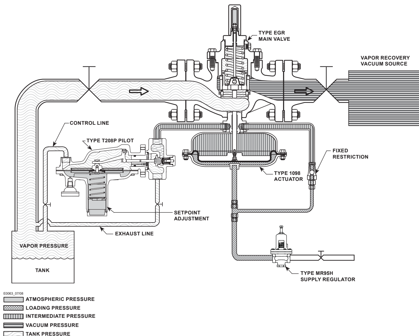
Figure 2. Operational Schematic
