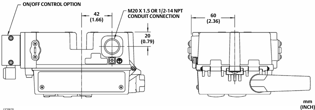
Figure 3. Dimensions—External Power Option
