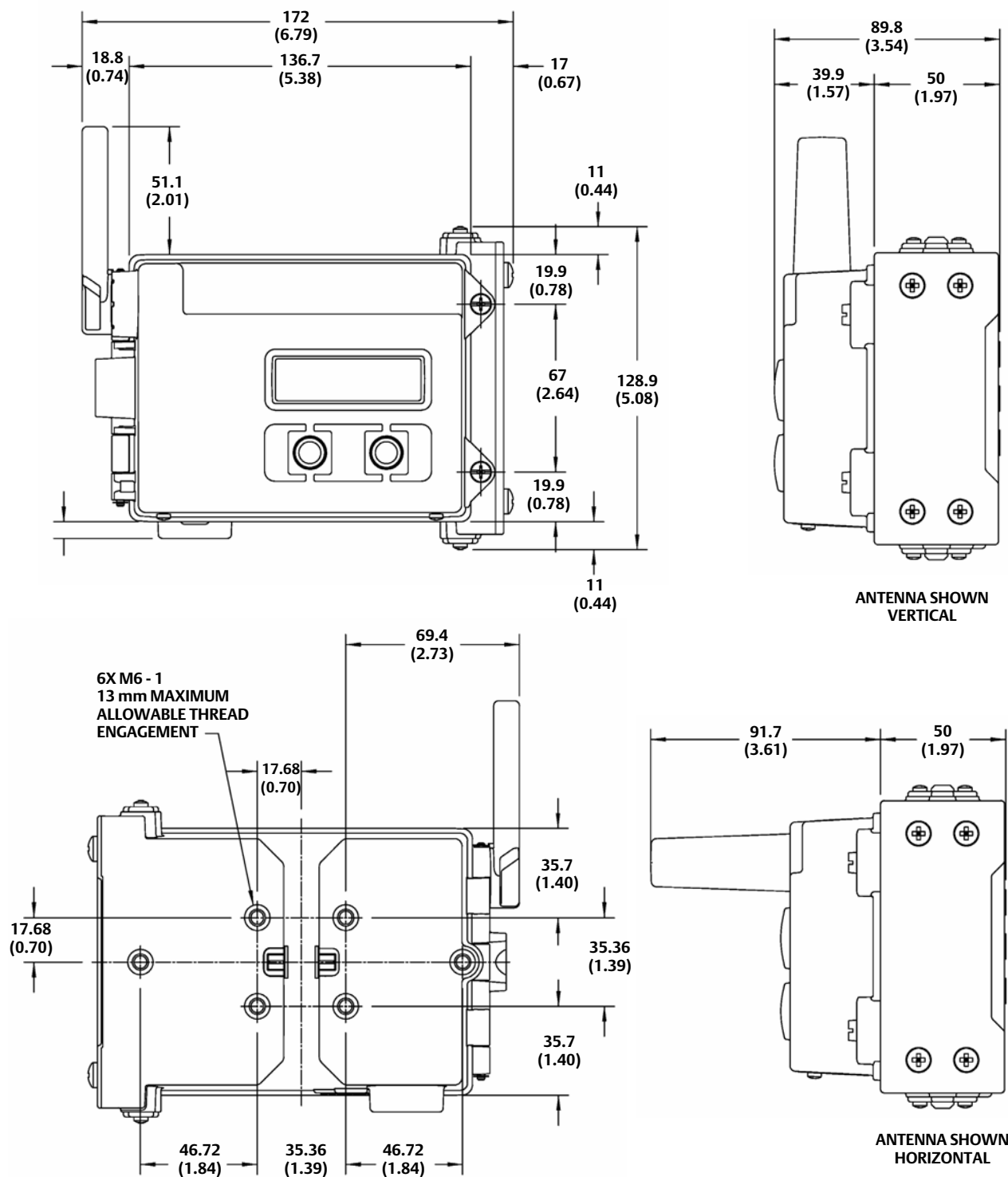
Figure 1. Dimensions
