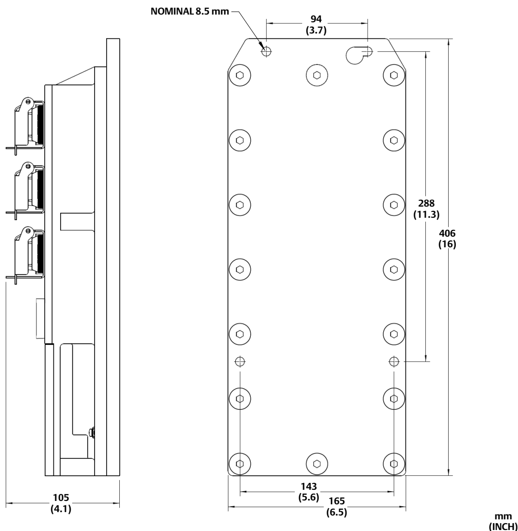
Figure 2. Dimensions
