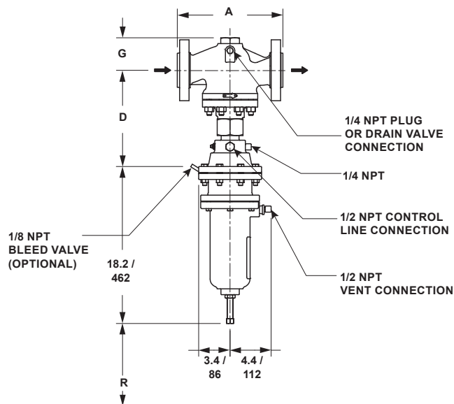
TYPE MR108 WITH HIGH-PRESSURE ACTUATOR
