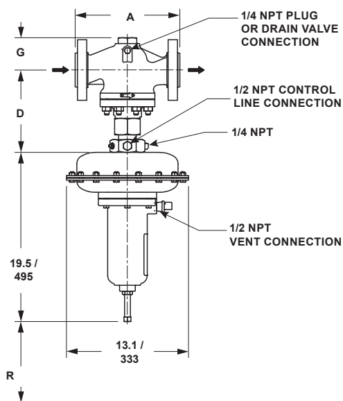
TYPE MR108 WITH LOW-PRESSURE ACTUATOR
