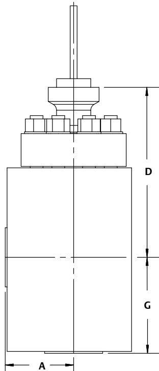
Figure 7. Typical CL2500 6-Stage NotchFlo DST Angle Valve Dimensions (also see table 24)
