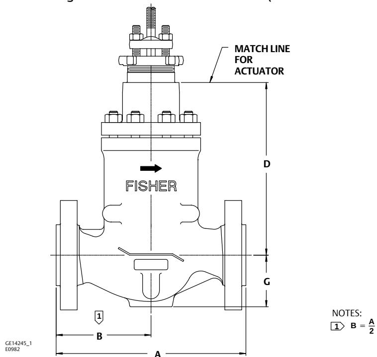
Figure 2. Typical CL300 and CL600 3-Stage NotchFlo DST Valve Dimensions (also see tables 13 and 14)
