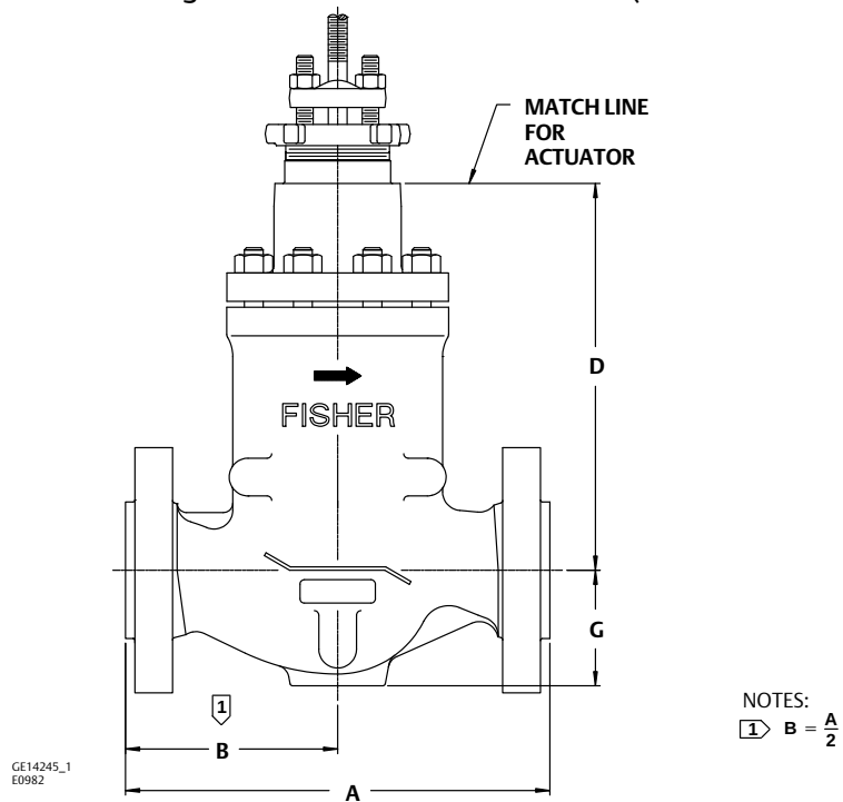
Figure 6. Typical CL1500 and CL2500 6-Stage NotchFlo DST Valve Dimensions (also see table 22 and 23)
