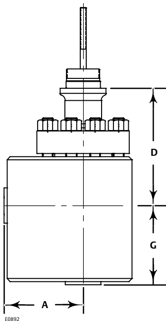
Figure 4. Typical CL300 3-Stage, CL600 3-Stage, CL900 4-Stage, and CL1500 4-Stage NotchFlo DST Angle Valve Dimensions (also see tables 17, 18, and 19)
