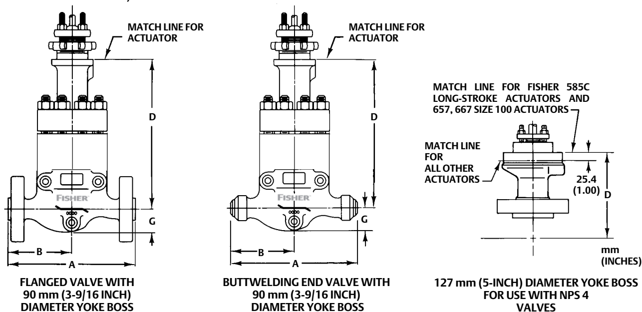
Figure 3. Typical CL900 and CL1500 ≤ NPS 4, 4-Stage NotchFlo DST Globe Valve Dimensions (also see tables 15 and 16)
