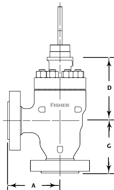
Figure 5. Typical CL1500 4-Stage NotchFlo DST Cast Angle Valve Dimensions (also see tables 20 and 21)
