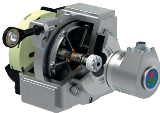
ROBUST, INDUSTRIAL VERSION FOR LARGE MEASURING LENGTHS UP TO MAX. 60.000 MM
