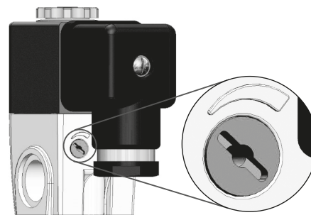
Fig. 5: Manual override
