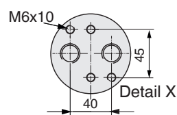
Type 2000U-4000U
