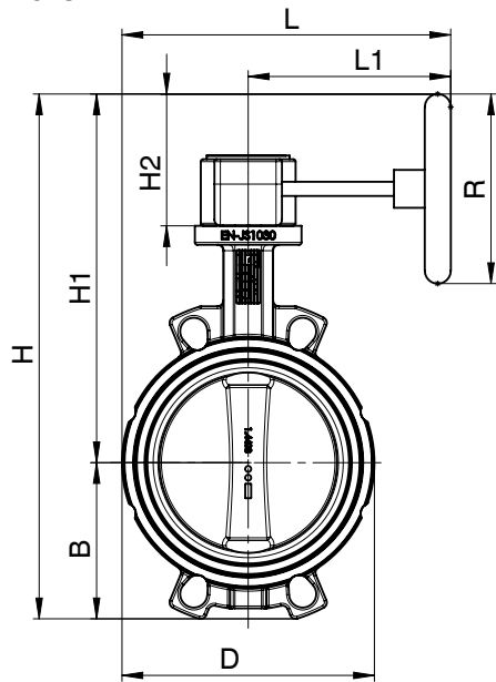
Wafer
