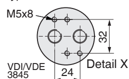
Type 2000U-4000U
