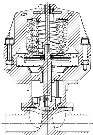
Sectional drawing
