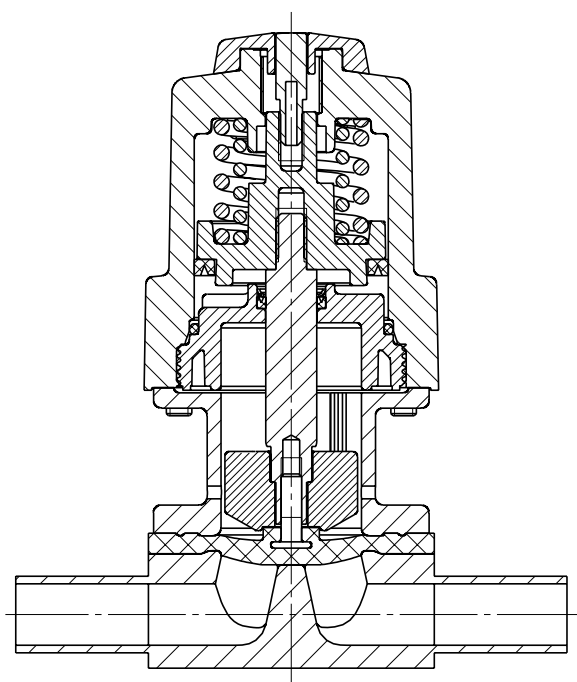
Sectional drawing
