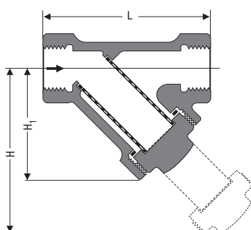
Y-type strainer with screwed connections series 330 GSF 331, PN 16, EN-JL 1040 GSF 332, PN 16, GP240GH GSF 333, PN 40, GP240GH GSF 334, PN100/160, GP240GH GSF 335, PN 40, CuZn39Pb3 GSF 337, PN 40, 1.4408 GSF 338, PN 100/160, 1.4408
