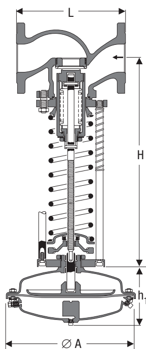
Pressure-reducing valve 5801
