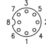
View from the bushing weld side
