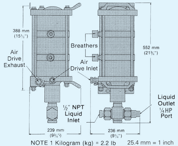
2 hp high ratio pumps; -683 and -903 ratios
