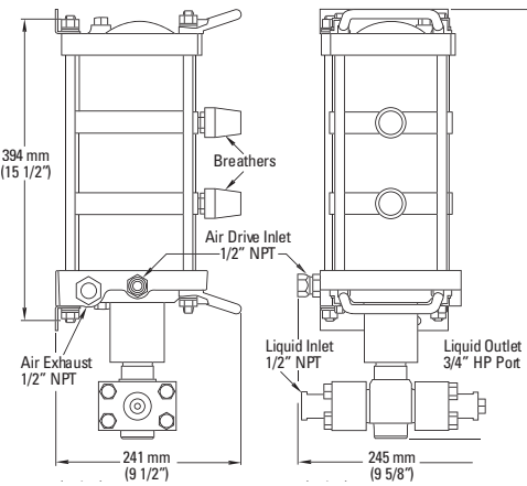
2 hp (1.49 & 1.64 kW) pump models; -1373 ratio
