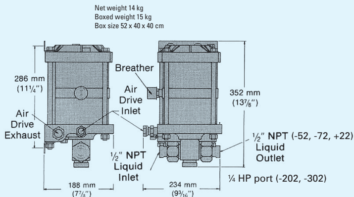
1.5 and 2 hp medium ratio pumps; -52, -72, -122, -202 and -302 ratios
