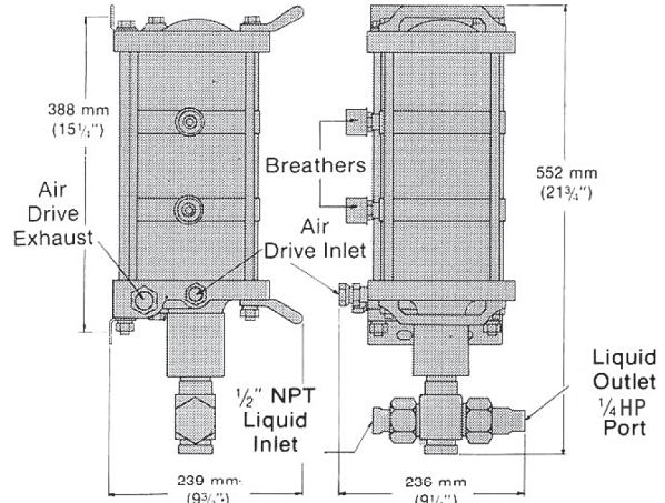
2 hp high ratio pumps; -683 and -903 ratios
