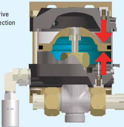
2. Hydraulic Check Valves
