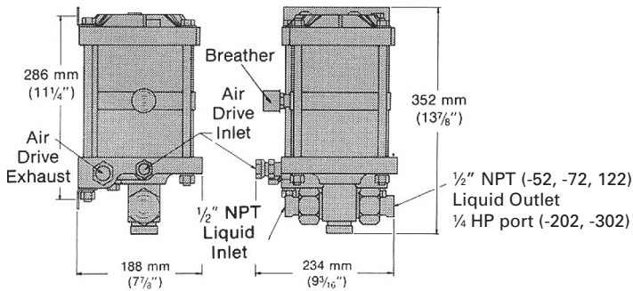
1.5 and 2 hp medium ratio pumps; -52, -72, -122, -202 and -302 ratios
