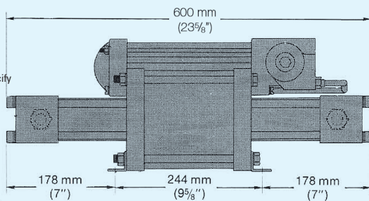
Models GWD, GSFD nominal ratio 12:1
