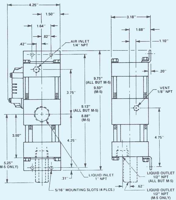
MDSTV-5, MDTV Approx weight 15 1/2 lbs (7 kg)
