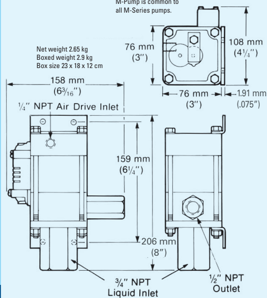
M-7, M-12 approx. weight 9 lbs (4 kg)
