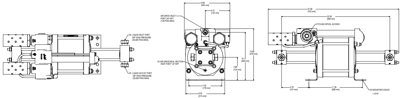
Model 8HSFD-25 Inlet, Outlet ports 3/8" HP
