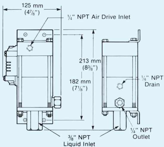
29723-21, 29723-36, 29723-71, 29723-110 approx. weight 6.5 lbs (3 kg)
