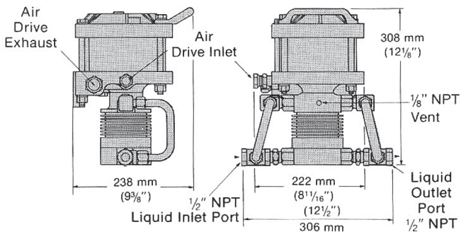
ATV-4 pumps; double acting, high output
