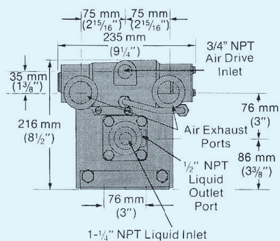
Models GW, GSF nominal ratio 35, 60 100:1
