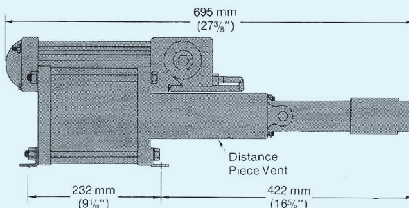
Models DGSF, DGSTV nominal ratio 35, 60 100:1
