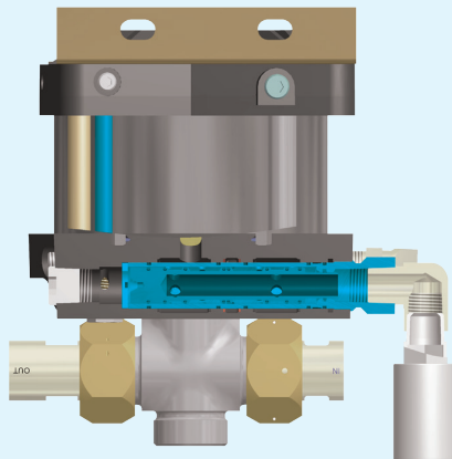
3. Drive Cycling Valve
