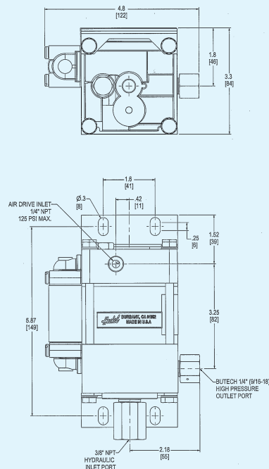
MS-220 approx. weight 6 lbs (2.7 kg)
