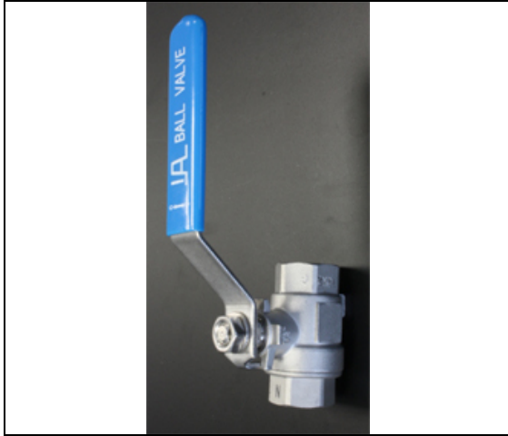
Fig. 20: Ball Valve PN 40 (580 psi); 1.4401 (316SS) (A56)
