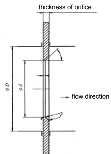
Fig. 7: Orifice plate for volumetric flow measurement
