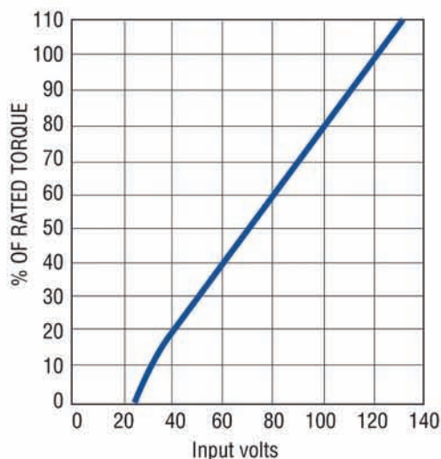
Typical Torque Versus Voltage for a Superior Motor
