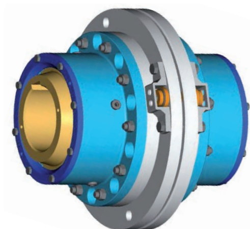
Gear Couplings with crush bolt and continuous oil lubrication
