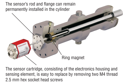
Fig. 2: Fluid cylinder installation with models RH, RF, GH (Only possible with sensors without the shock and vibration option.)
