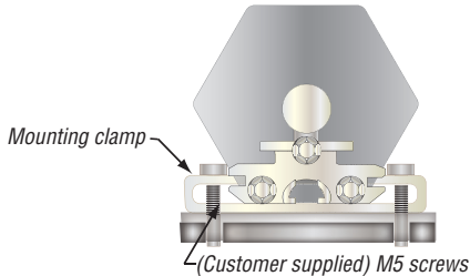
Fig. 5: Mounting clamp and screws
