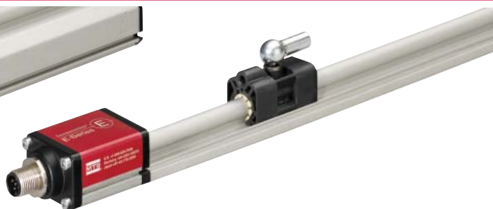
Model EL position sensor - Low Height Profile Housing Stroke Length: 50 mm to 2500 mm (2 in. to 100 in.)
