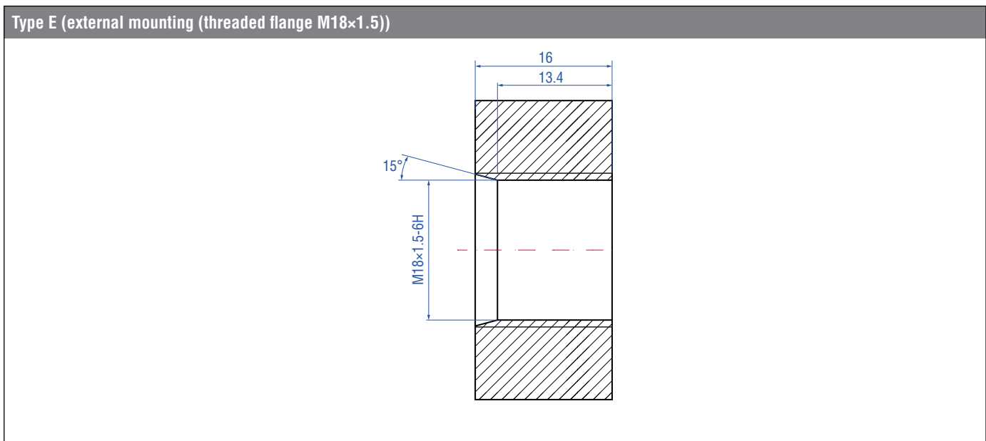
Fig. 20: Internal thread in cylinder
