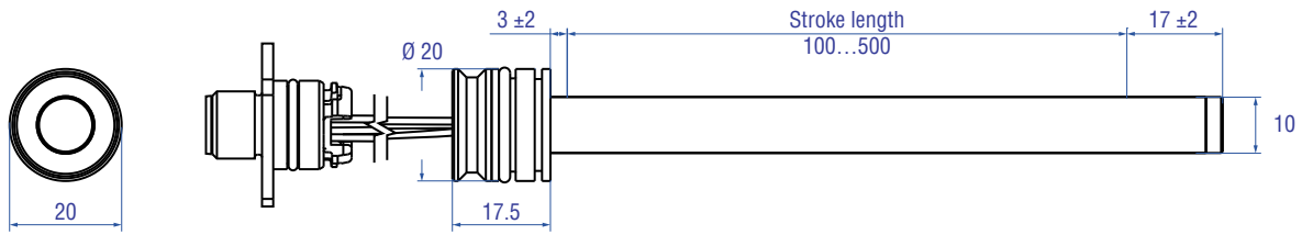
Fig. 17: HE Sensor Type D
