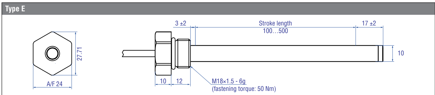
Fig. 19: HE Sensor Type E
