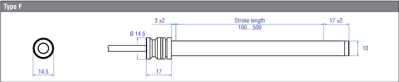
Fig. 21: HE Sensor Type F
