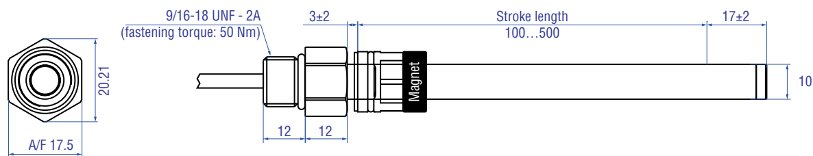
Fig. 11: HESensor Type A
