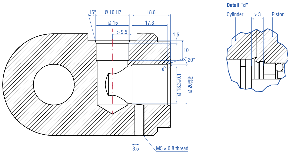
Fig. 18: Cavity fit in cylinder
