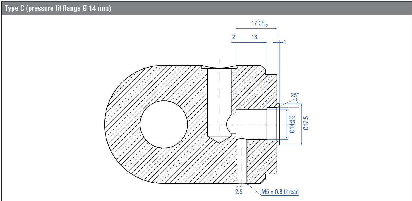
Fig. 16: Cavity fit in cylinder
