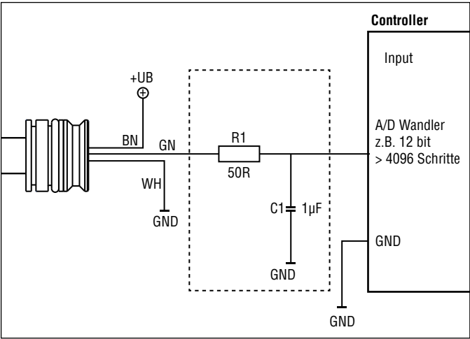
Fig. 36: Noise reduction
