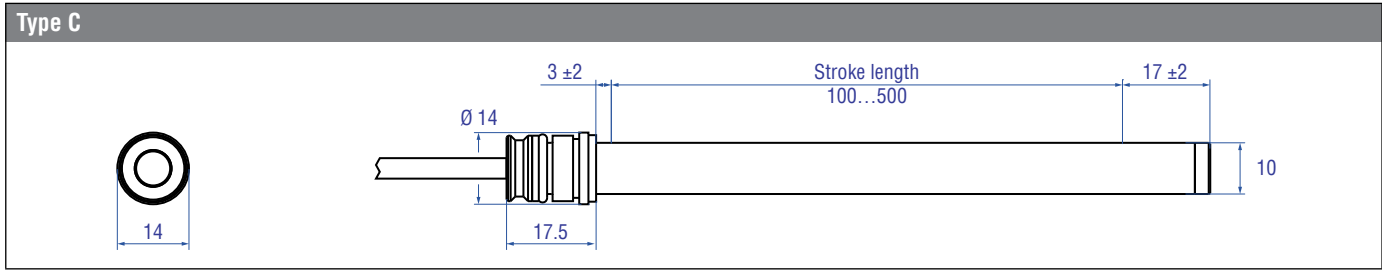
Fig. 15: HE Sensor Type C
