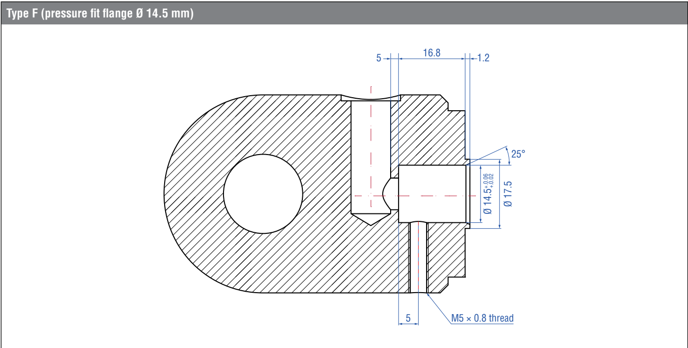
Fig. 22: Cavity fit in cylinder
