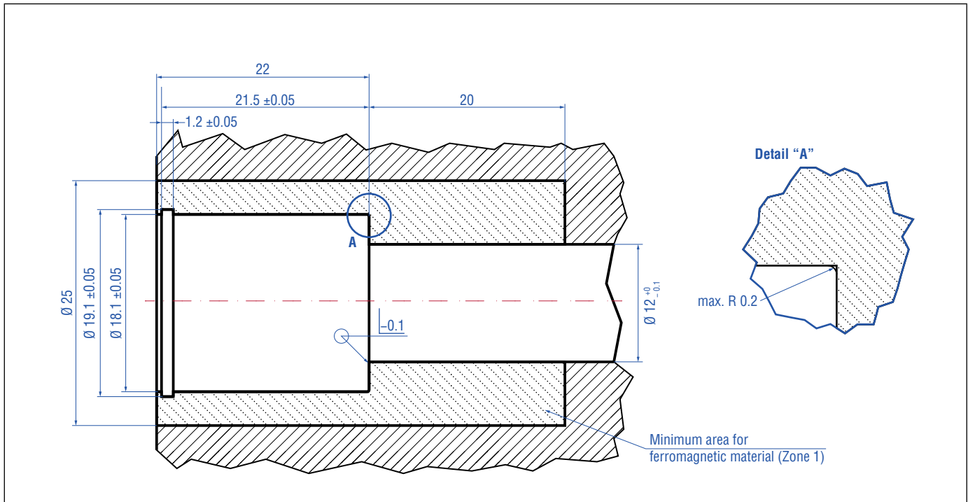
Fig. 6: Ferromagnetic material
