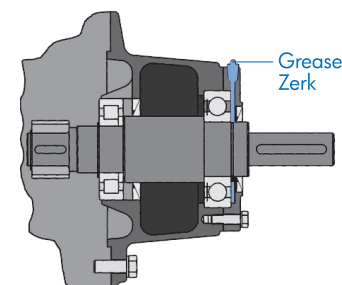
Re-Lubricating the bearing with the Grease Zerk
