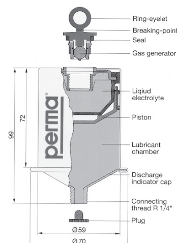
Automatic Lubricator Dimensions & Descriptions
