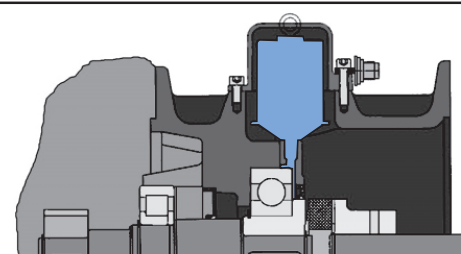
Automatic Lubricator
