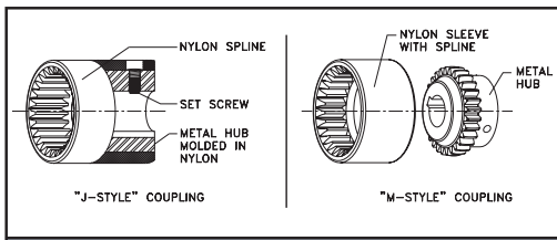
J & M Style Coupling Illustrations
