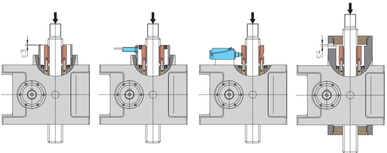
Thread wear control on screw jacks MA Series Mod.A
