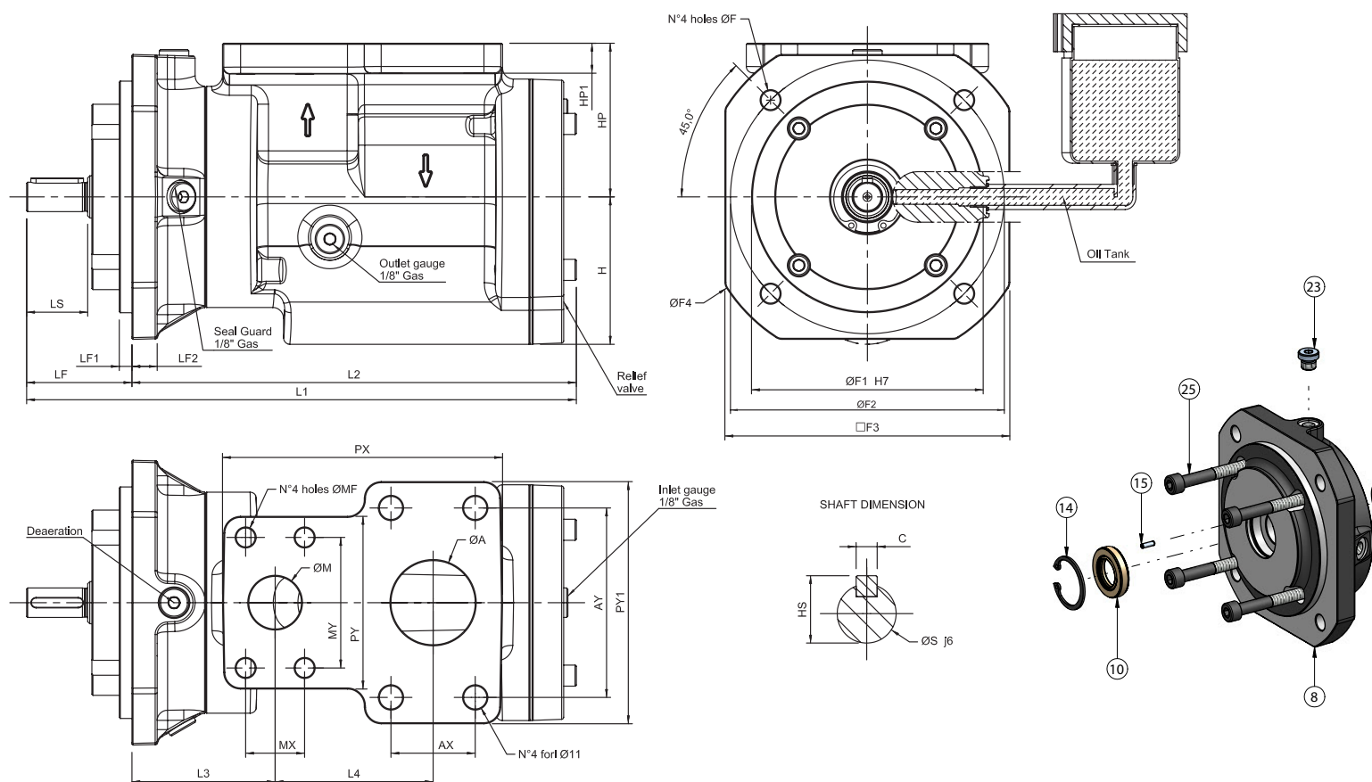
Pump / Pompa
