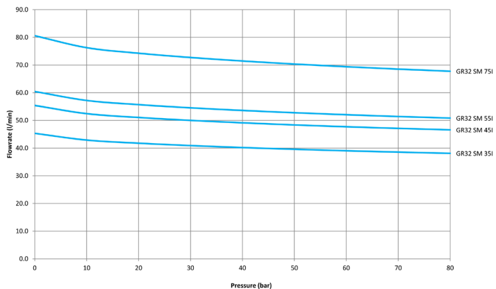
Flowrate GR32 SM @ 2750 RPM - 68 cSt
