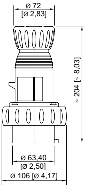
5-pole plug
