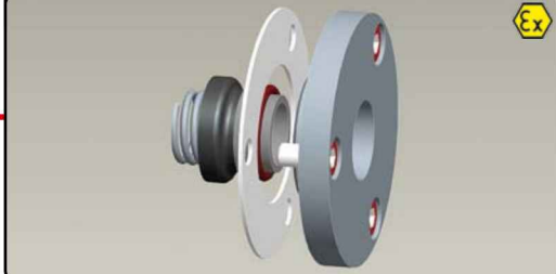
Mechanical seal GLRD
