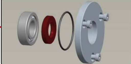
ball bearing with radial shaft seal KR
