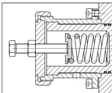
construction D (pressure relief valve)
