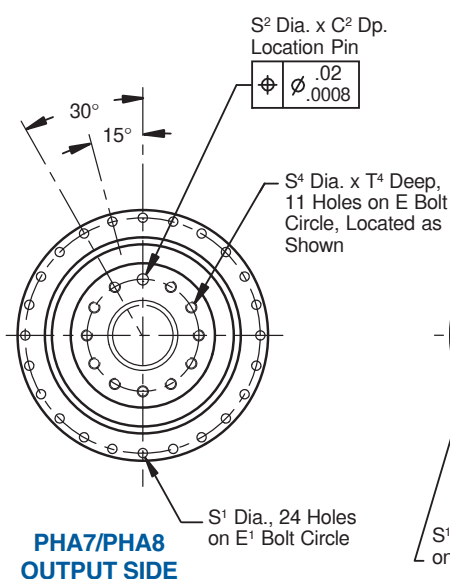
"PHA" Series – Advanced Gearhead with Motor Plate – Dimensions (mm/inches)
