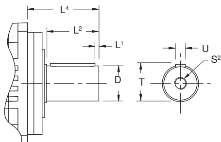
"P" – Shaft with Key
