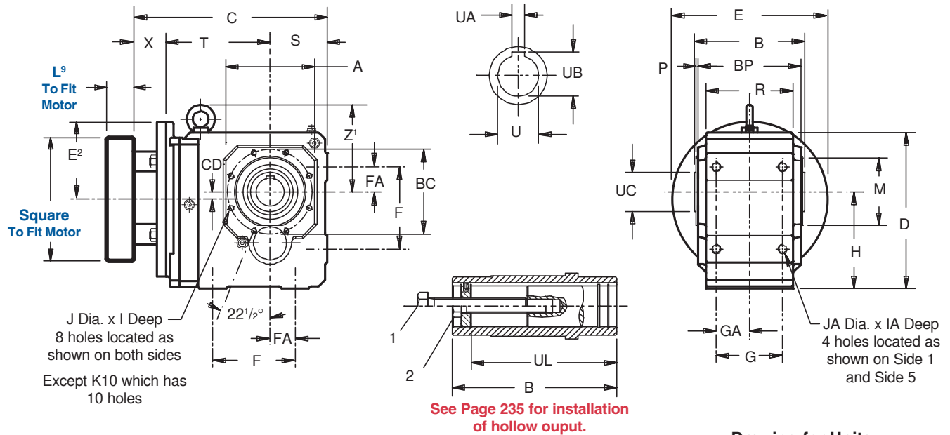
Drawing for Units K513AG — K1014AG
