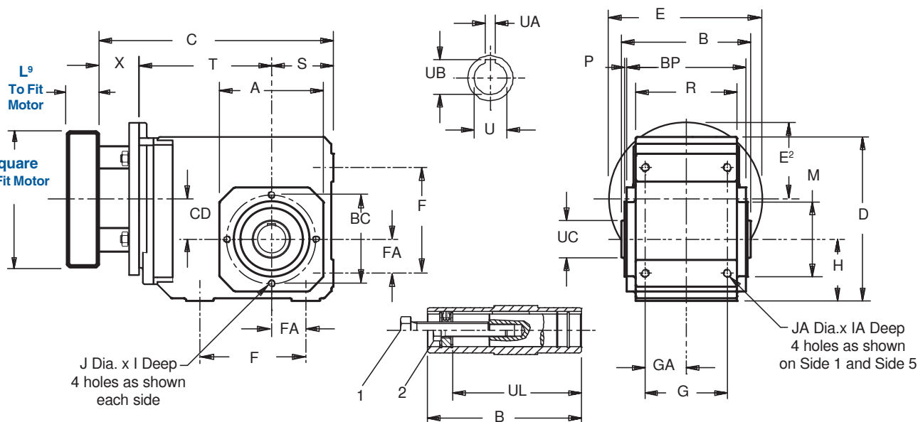
Drawing for Units K102AG — K403AG
