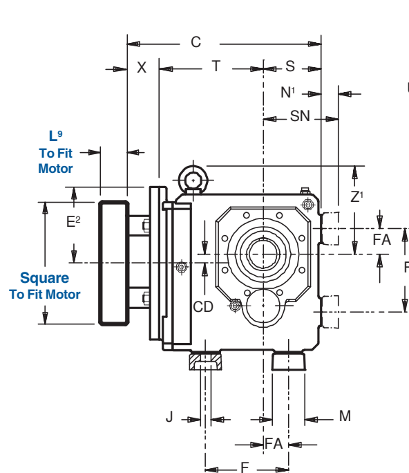
Drawing for Units K513VN — K1014VN
