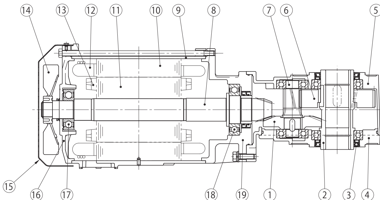
Figure C1 LNYM8-HZ523-EP
