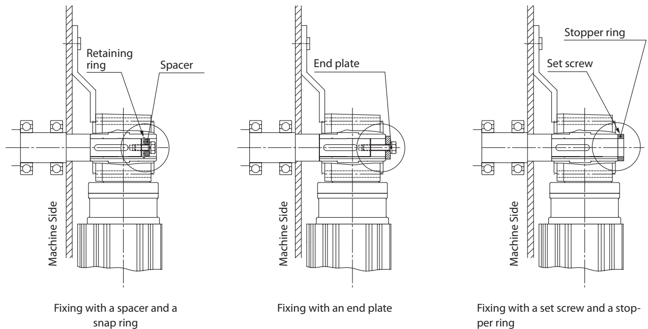
Figure C7 Fixing methods in which the present product does not move to the opposite of the machine.
