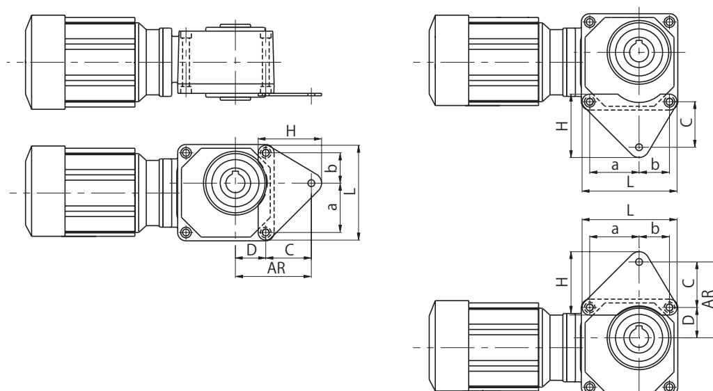
Figure C13 Installation example
