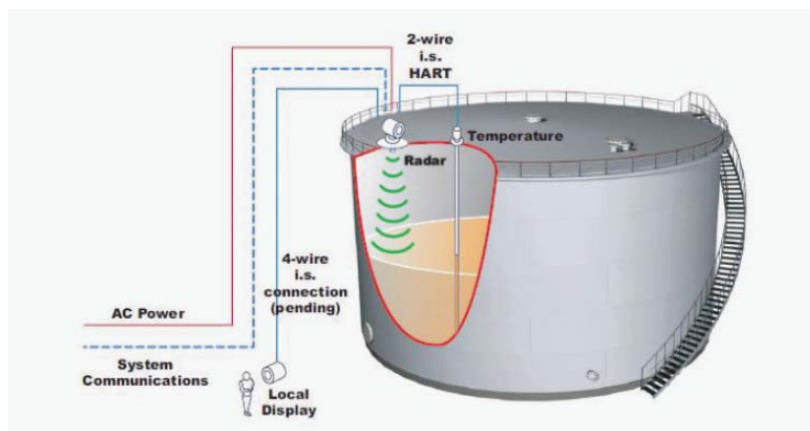
Example Tank Gauging System
