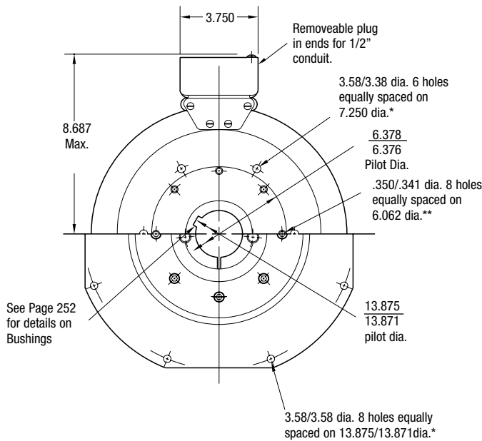
FIELD VIEW
