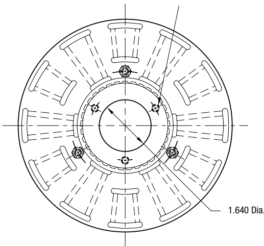
ARMATURE VIEW
