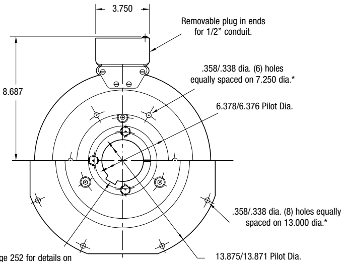
MAGNET VIEW
