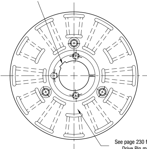
ARMATURE VIEW
