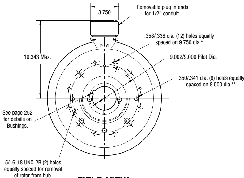
FIELD VIEW
