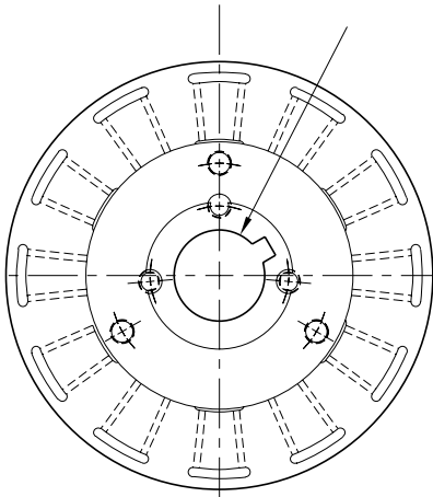
ARMATURE VIEW
