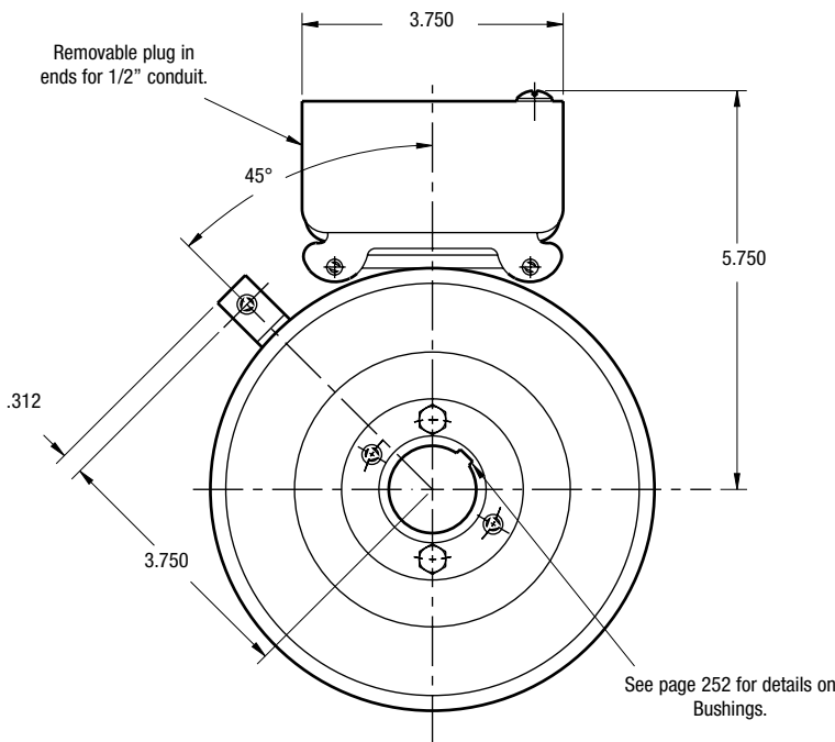
FIELD VIEW
