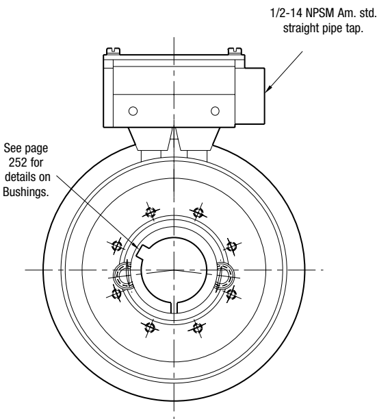
MAGNET VIEW
