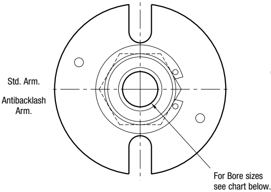
ARMATURE VIEW
