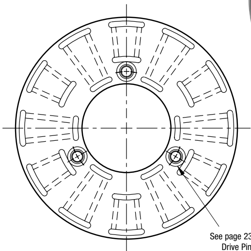
ARMATURE VIEW
