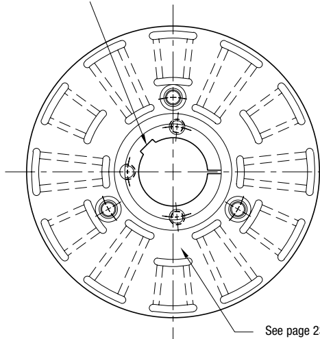
ARMATURE VIEW
