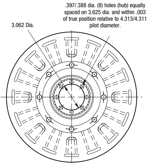
ARMATURE VIEW
