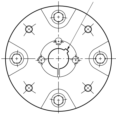
HUB VIEW
