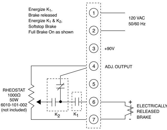
Soft Stop for Electrically Released Brake
