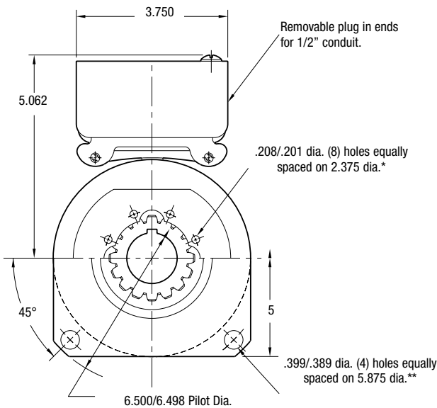
MAGNET VIEW
