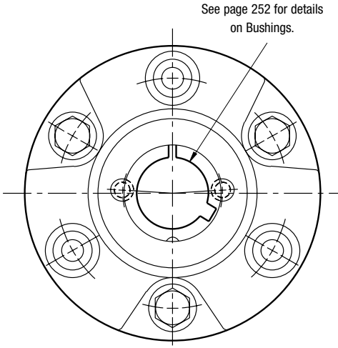
HUB VIEW
