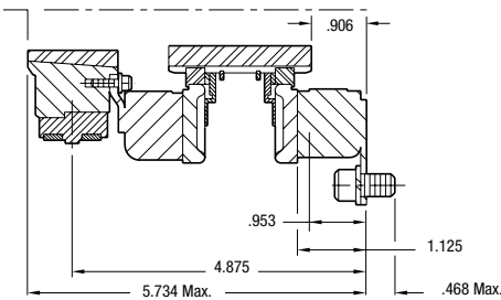
Outside Mounted Flush Backing Plate
