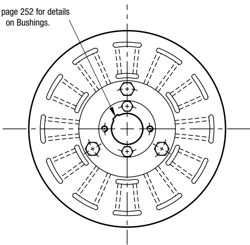
ARMATURE VIEW
