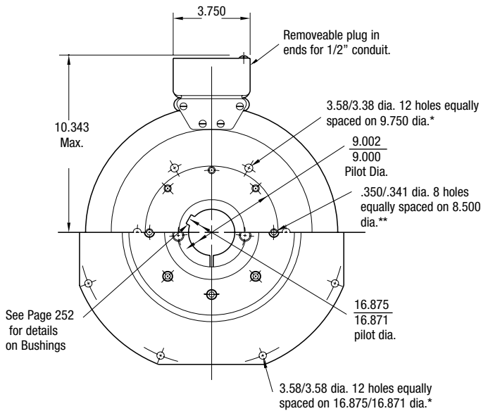
FIELD VIEW
