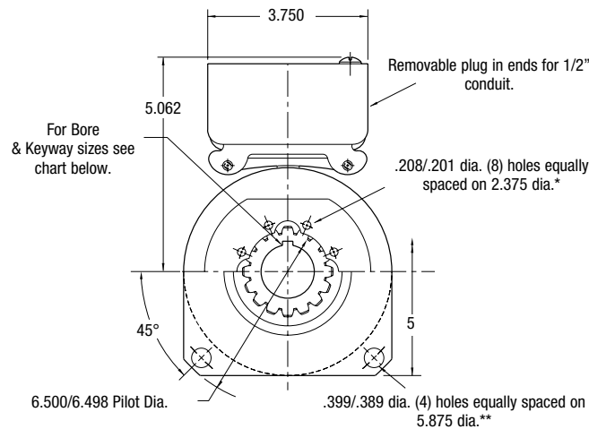
MAGNET VIEW
