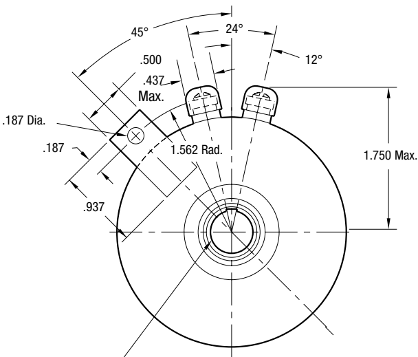
ARMATURE VIEW
