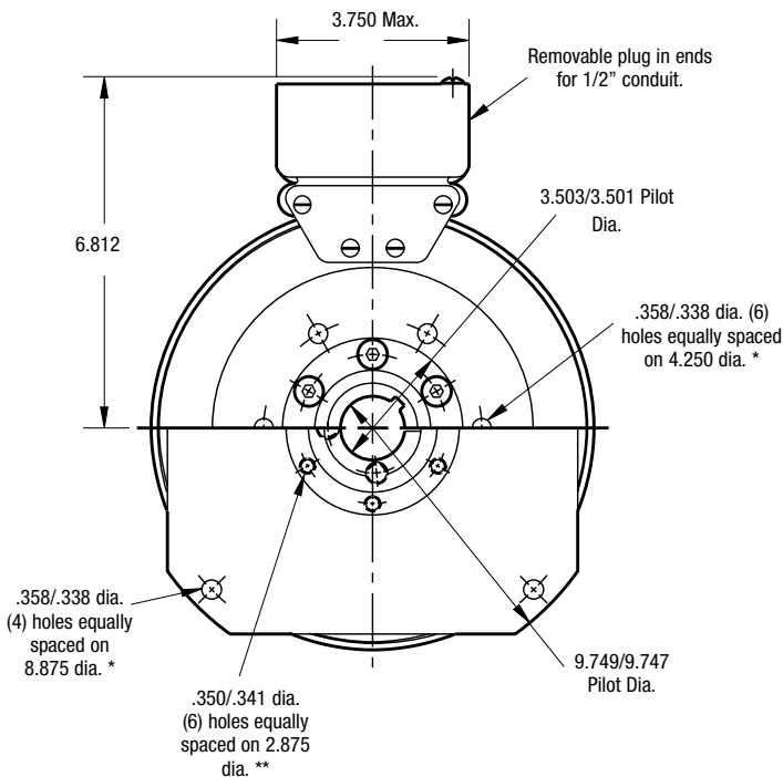
FIELD VIEW
