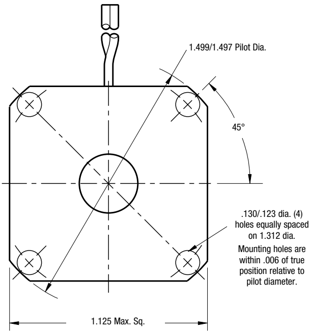
MAGNET VIEW
