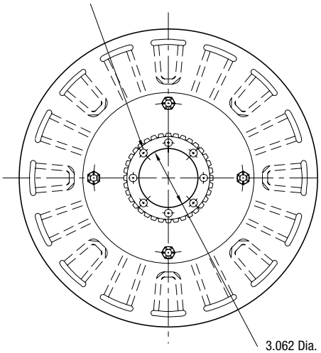
ARMATURE VIEW
