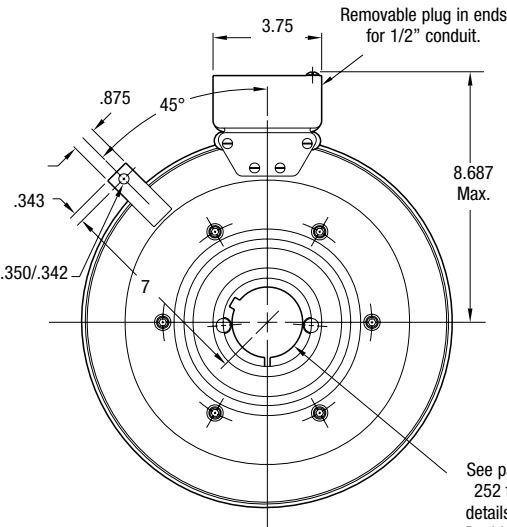
FIELD VIEW
