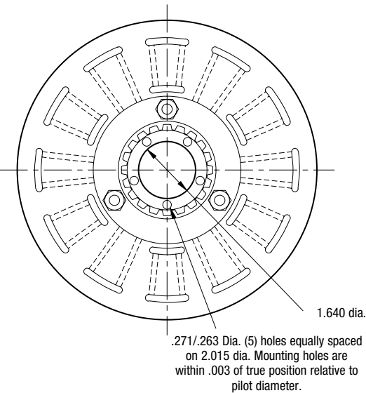
ARMATURE VIEW
