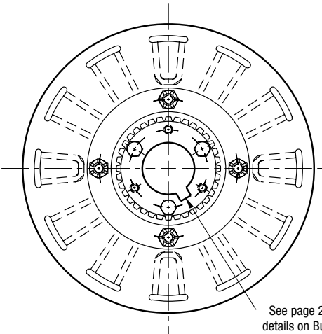
ARMATURE VIEW
