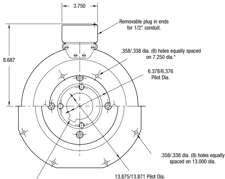
ARMATURE VIEW
