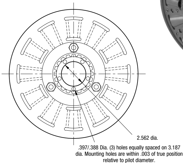
ARMATURE VIEW
